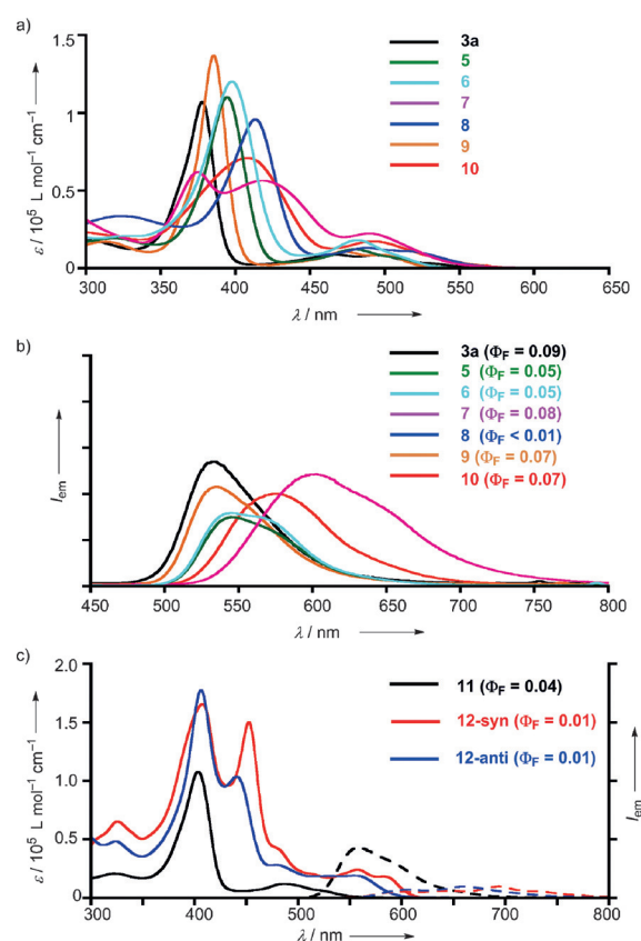
Figure 2. a) UV/Vis absorption and b) fluorescence spectra of subporphyrins 3a and 5–10 in CH 2 Cl 2 and c) UV/Vis absorption (—) and fluorescence (----) spectra of subporphyrins 11 , 12-syn , and 12-anti in CH 2 Cl 2 .
